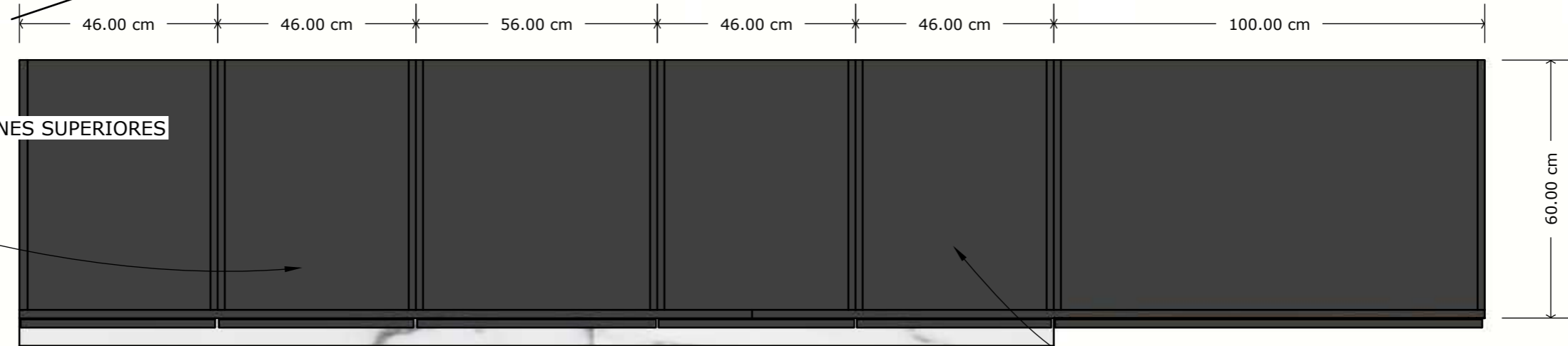
VISTA FRONTAL
